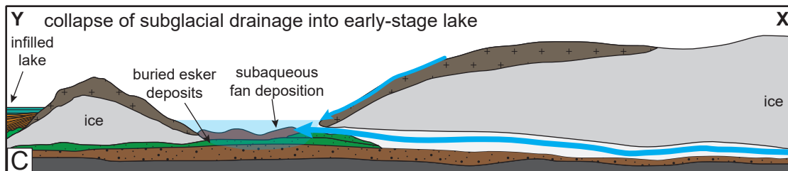
Figure 9 – Conceptual model showing formation of North Scales ice-walled lake plain and esker ridges based on interpretation of GPR data. (A) Brampton Kame Belt conceptual model, adapted from Livingstone et al. (2010c). Panels (B) to (F) are two-dimensional cross-sections showing the evolution of a section of the kame belt along the transect X-Y, which transitions from a major subglacial drainage channel into an ice-walled lake. The situation depicted in (A) is broadly equivalent to that shown in panels (C) and (D) in terms of stage of kame belt evolution. (B) Ice sheet with major subglacial drainage axis and late-stage ice-walled lake forming. (C) Partial collapse of drainage axis into early-stage lake as glacier karst begins to develop. (D) Lake expansion as glacier karst evolves. (E) Late-stage lake infill and esker formation. (F) Esker ridges and ice-walled lake plains.
